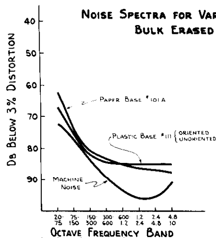
Figure 3. Bulk erased noise spectra for the same tapes as in Figure 2. The machine noise (tape motion stopped) is also shown.
