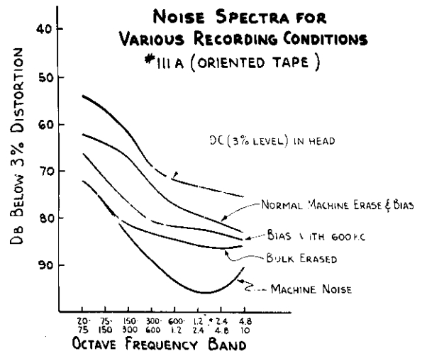
Figure 4. Noise spectra showing the effect of various erasure conditions.
