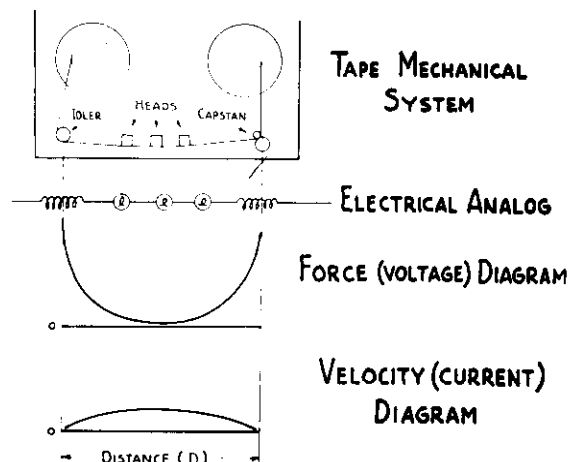
Figure 1. Diagram showing the mechanical drive parts of a tape recorder. Longitudinal tape vibrations are excited by friction with the heads and exhibit an amplitude pattern as shown.
