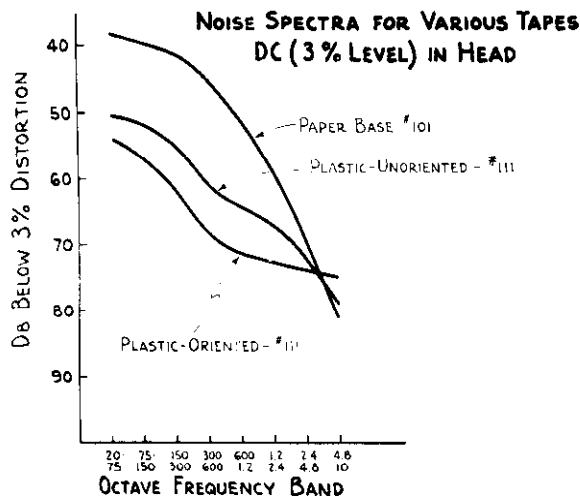
Figure 2. DC noise spectra for paper base tape and plastic base tapes with and without particle orientation. Tape speed 7.5 ips. NARTB playback equalization.
